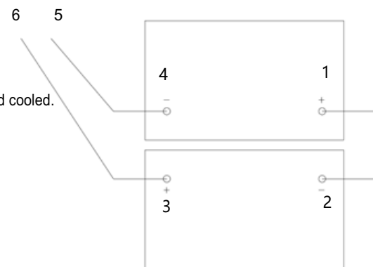
Figure 7-1 Battery main power wiring diagram
